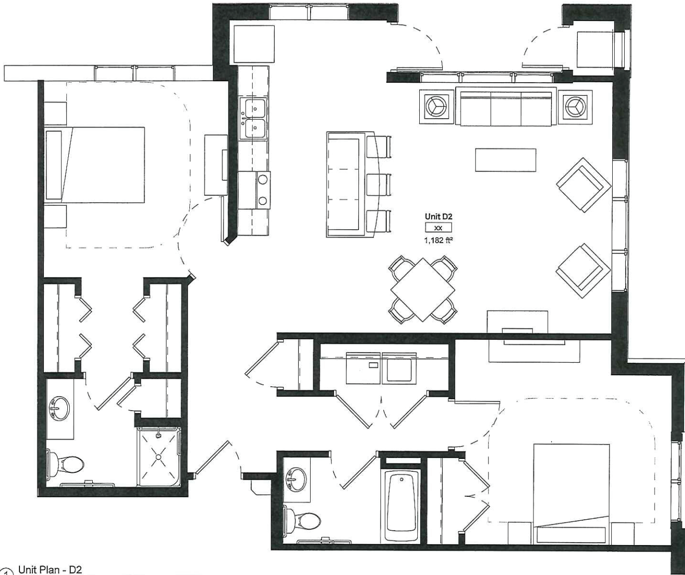
① Unit Plan - D2 1/4" = 1'-0"
