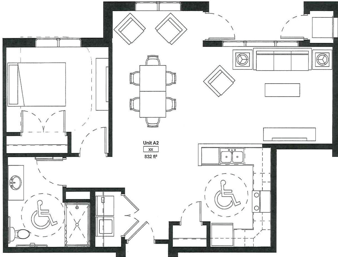
① Unit Plan - A2 1/4" = 1'-0"
