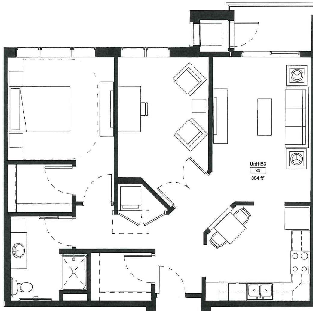
① Unit Plan - B3 1/4" = 1'-0"
